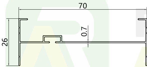
DOUBLE JAMB Weight: 0.269kg/m
