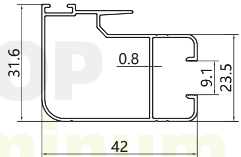
INTERLOCKER Weight: 0.372kg/m
