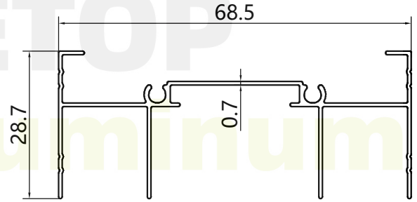
DOUBLE HEAD Weight: 0.378kg/m
