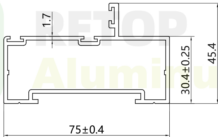
RG1206151 WEIGHT : 1.154kg/m
