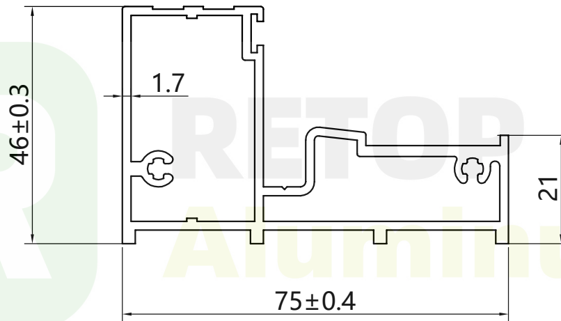
RG1206150 WEIGHT : 1.422kg/m
