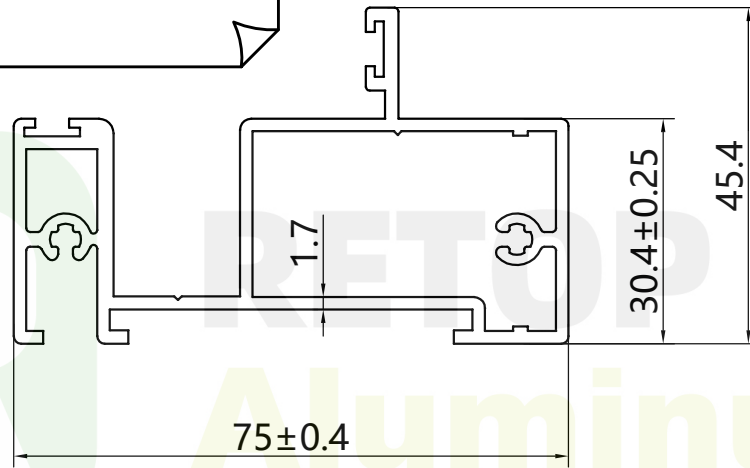
RG1206149 WEIGHT : 1.411kg/m
